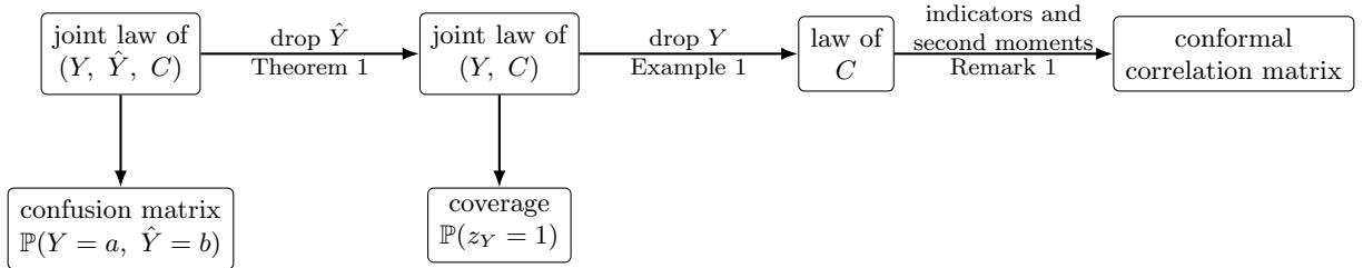
Figure 1: The chain of coarsenings from the data to the matrix. The confusion matrix is a function of the first object. Theorem 1 shows it is already lost at the first step, where the ranked prediction is dropped. Example 1 shows a further loss of one bit at the second step, where the true label is dropped. The coverage guarantee constrains one scalar of the second object. The matrix is a function of the third.
