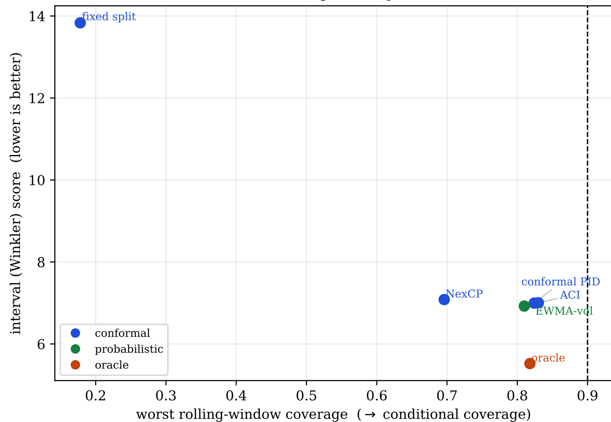
The coverage--score plane
