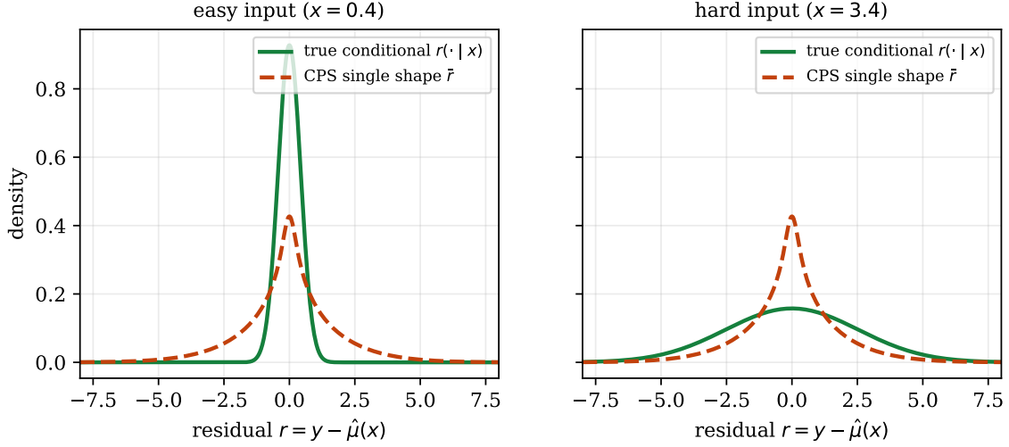
Figure 5: The residual-information gap (Propositions 2–3). A single-shape conformal predictive system uses the marginal residual law \tilde{r} for every input; the oracle uses the true conditional r(\cdot | x) , narrow for easy inputs (left) and wide for hard ones (right). The expected log-score regret is exactly the mutual information I(R; X) , which no X -ignoring recalibration can reduce.
