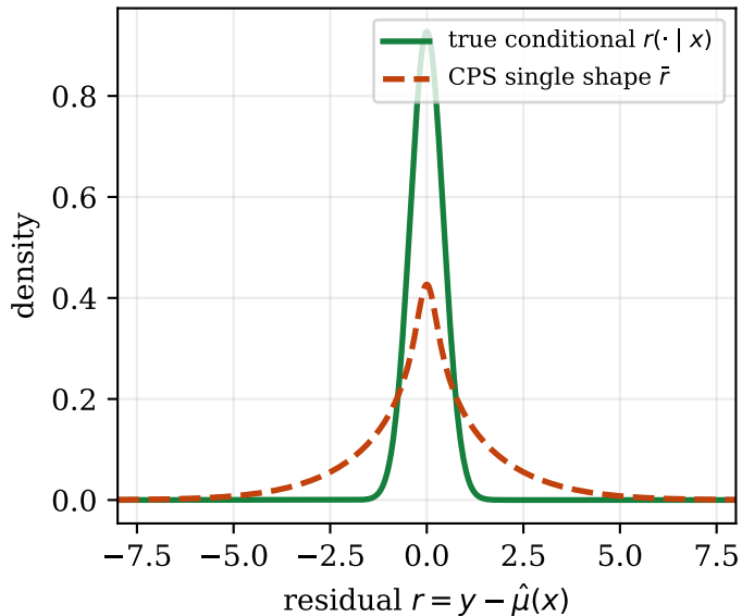
easy input ( x = 0.4 )
