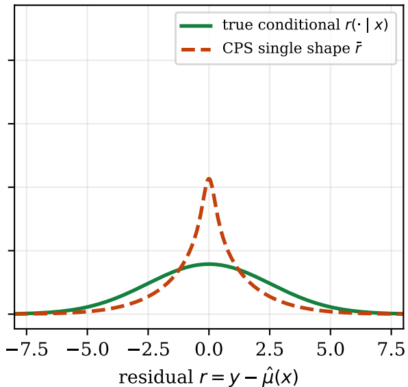
hard input ( x = 3.4 )
