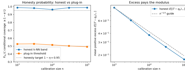
Figure 3: Lognormal scores at the smooth baseline, \eta = 0.05 . Left: the honesty probability, the probability over calibration samples that the realized threshold attains conditional coverage at least 1 - \alpha . The honest k -nearest-neighbour band (7) clears the target 1 - \eta = 0.95 . The uncorrected plug-in meets it on about half the samples. Right: the honest band’s positive excess \mathbb{E}[(T - q_\alpha)_+] , decaying at the predicted n^{-1/3} .
