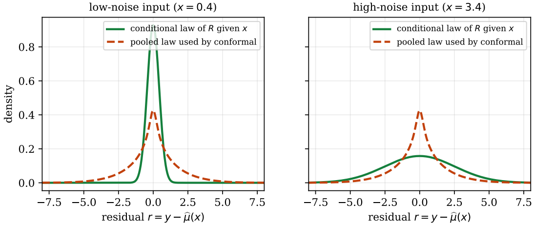
Figure 1: The conformal information gap when the error spread grows with the input. A single-stratum conformal scheme uses the pooled law (dashed) for every input. It is too wide for low-noise inputs and too narrow for high-noise ones. Its excess log loss over the conditional law (solid) is I(R; X) , here 0.243 nats per observation.
