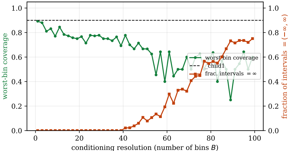
The price of conditional coverage (Lemma 1a)
