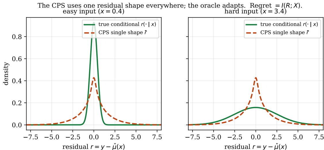
Figure 5: The residual-information gap (Propositions 2–3). A single-shape conformal predictive system uses the marginal residual law \bar{r} for every input; the oracle uses the true conditional r(\cdot | x) , narrow for easy inputs (left) and wide for hard ones (right). The expected log-score regret is exactly the mutual information I(R; X) , which no X -ignoring recalibration can reduce.
