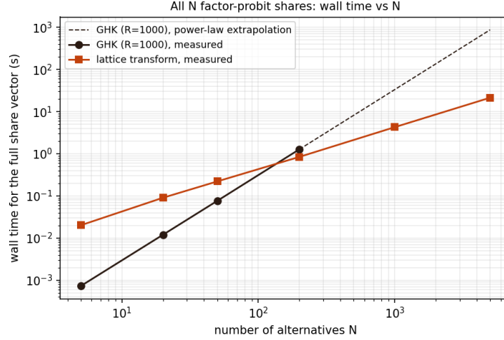
Figure 1: Wall time for the full N -alternative share vector as N grows ( k = 2 factors). Measured points for both methods; dashed line is the power-law extrapolation of the per-alternative GHK cost at R = 1000 , at which setting its error is \sim 10^{-3} against the lattice’s \sim 3 \times 10^{-4} (Table 1). Matched-accuracy GHK cost at N = 5000 extrapolates to \sim 40 hours (Section 2).
