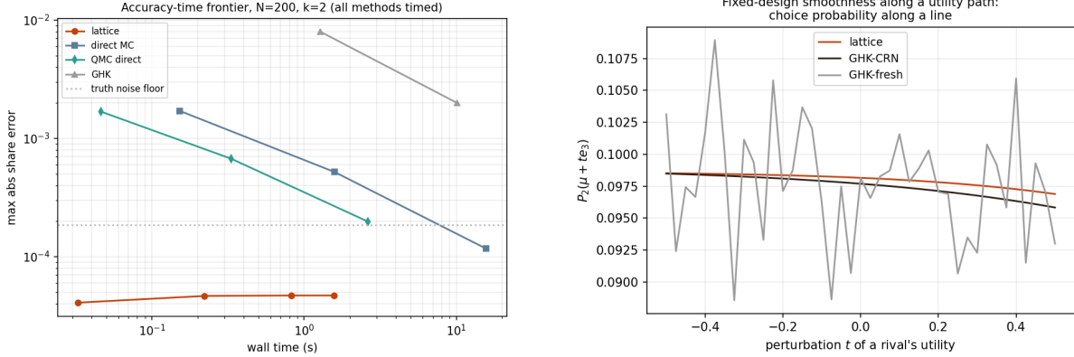
Figure 2: Left: measured accuracy–time frontier at N = 200 , k = 2 (experiment 17) — every method timed on the same problem against twin 5 \times 10^7 -draw references; direct simulation is a first-class baseline. Right: fixed-design smoothness along a utility path. Fresh-draw GHK shows run-to-run simulation noise (roughness statistic — maximum second difference over dt^2 — 39.3, versus 0.01 for both common-random-number GHK and the lattice); CRN-GHK is smooth conditional on its draw set, and the offset between its curve and the lattice’s is a discrepancy between two approximations; decomposing it requires an independent high-accuracy reference. All three curves are approximations.
