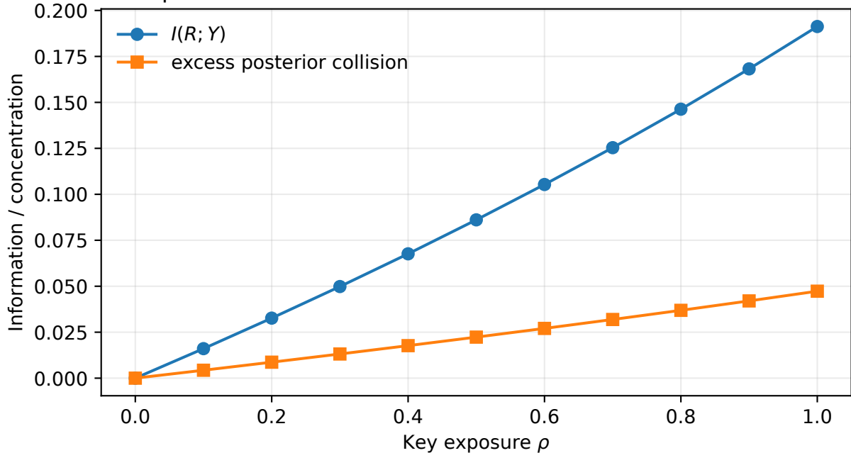
More exposed Gaussian factor means more evidence and less diversity
