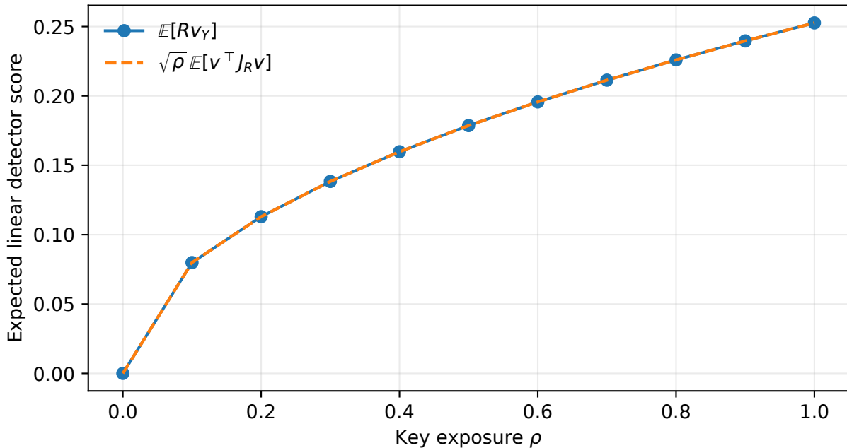
Stein identity for the model-free Gaussian detector
