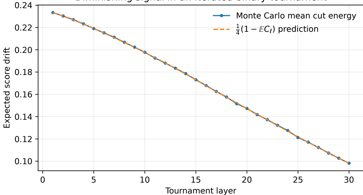
Diminishing signal in an iterated binary tournament
