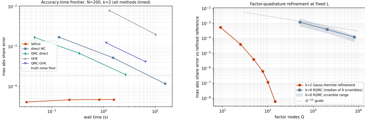
Figure 2: Left: each method at its most accurate tested setting, timed on the same N = 200 , k = 2 problem against one common reference (twin 5 \times 10^7 -draw simulations; experiment 17). The shaded band is the reference’s own noise: the lattice point sits at that floor, and its true error is \sim 10^{-8} by self-convergence. Right: factor-quadrature refinement at fixed L : Gauss–Hermite at k = 2 , and at k = 8 the median and range over eight independent RQMC scrambles.
