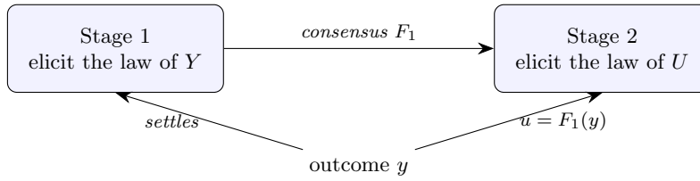
Figure 1: A residual chain. Stage 1's consensus F_1 becomes the frame for stage 2, which settles on the transformed outcome u = F_1(y) ; the same realized y anchors both. The base pool and its z_1 calibration stream are an instance.
