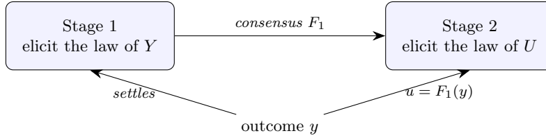
Figure 1: A residual chain. Stage 1's consensus F_1 becomes the frame for stage 2, which settles on the transformed outcome u = F_1(y) ; the same realized y anchors both. The base pool and its z_1 residual stream are an instance.
