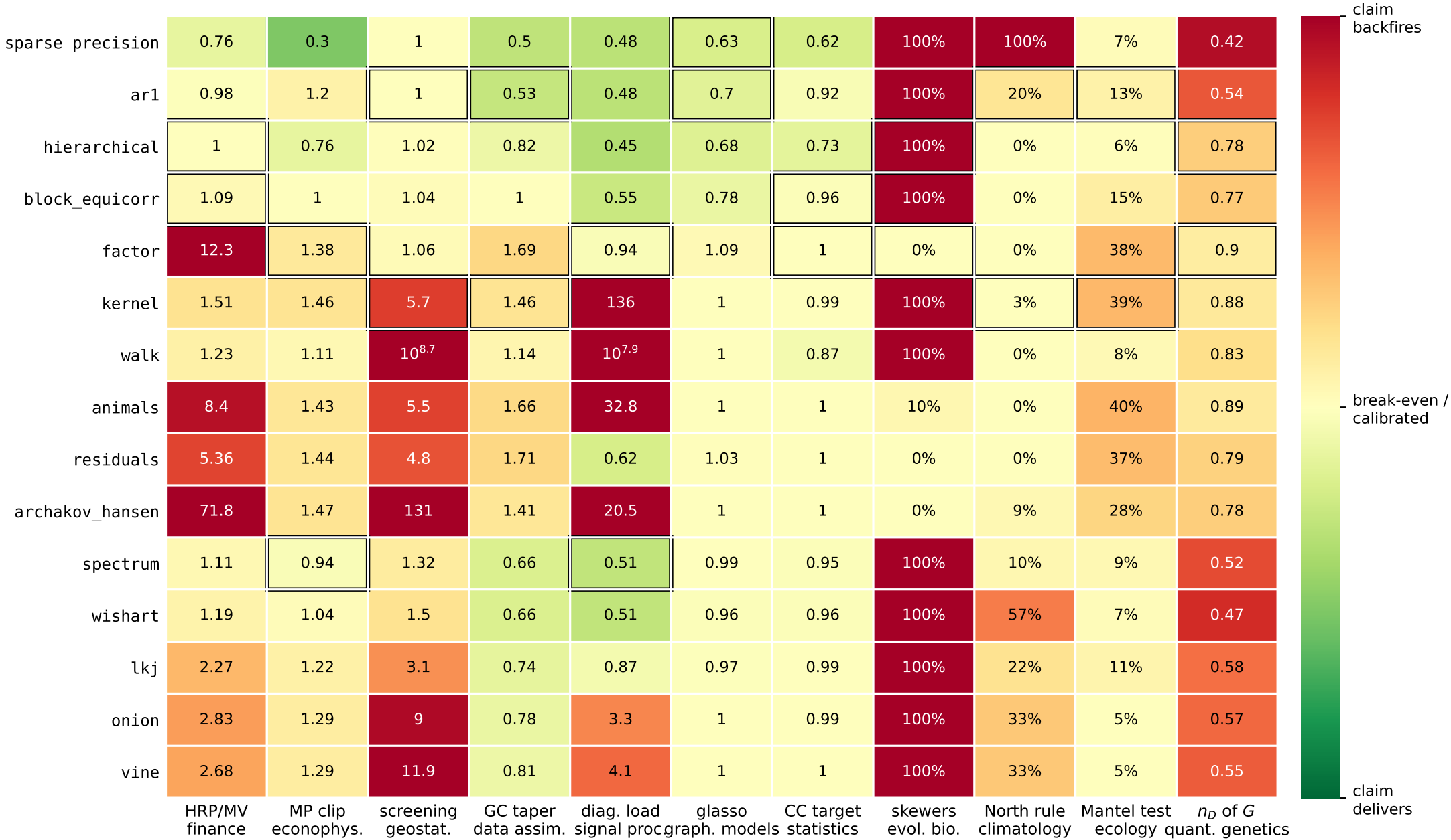
Eleven covariance-method claims across fifteen generating ensembles (outlined cells: the correlation structure the claim was demonstrated on or intended for)
