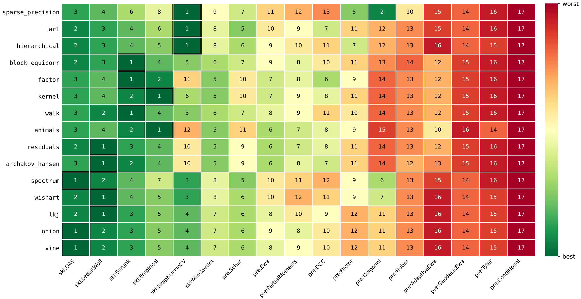
Rank of seventeen covariance estimators by generating ensemble (median relative Frobenius loss, n = 30 , T = 60 ; outlined cells: rank 1)
