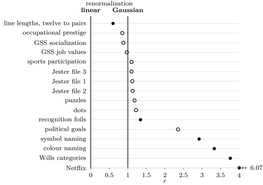
Figure 1: Where each population sits between the two maps. The coordinate is r = \lambda_{\text{observed}}/\lambda_{\text{Case V}} , the observed contraction slope divided by the slope Case V implies for that population’s own shares, so linear renormalization is at r = 0 by construction and Gaussian renormalization at r = 1 . Filled circles are restricted menus the observer actually faced, open circles are ranking-induced. Most populations lie beyond r = 1 : choice contracts by more than Case V predicts, so the Gaussian point is not far enough along the family, which is the same signed error the after-stimulus arms and Table 9 report. The one population on a perceptual continuum falls short of it instead. Sixteen of the thirty-nine comparisons appear; the others restrict to sets of three or more, so no pairwise q_{ij} exists and no slope can be fitted, which excludes the tone matrices, the Getty conditions and Townsend and Landon. Positions here do not reproduce Table 1: \lambda projects a vector of pair-specific predictions onto a single slope and is not a proper score, so the twelve-line population sits nearer Case V on this axis while linear renormalization has the lower held-out log loss on it. This axis places populations, the table scores forecasts. Netflix has three alternatives and three pairs.
