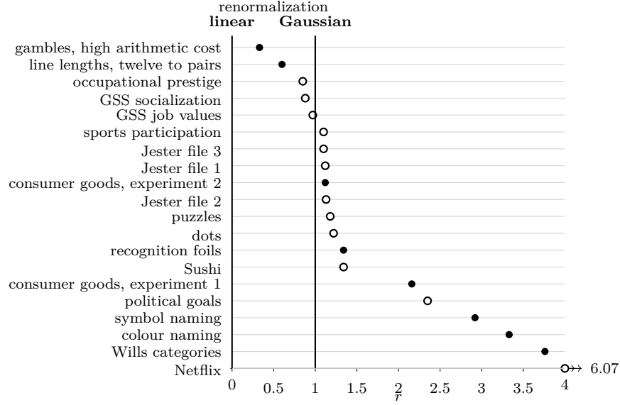
Figure 1: Where each population sits between the two maps. The coordinate is r = \lambda_{\text{observed}} / \lambda_{\text{Case V}} , the observed contraction slope divided by the slope Case V implies for that population’s own shares, so linear renormalization is at r = 0 by construction and Gaussian renormalization at r = 1 . Filled circles are restricted menus the observer actually faced, open circles are ranking-induced. Most populations lie beyond r = 1 : choice contracts by more than Case V predicts, so as a general observation the Gaussian point tends not to be far enough along the family. A collection appears when a restricted pairwise share q_{ij} exists on the alternatives that calibrated the map, which twenty of the thirty-nine comparisons have. The tone, Getty and Townsend rows restrict to sets of three or more, so no q_{ij} exists; the news, ballot and Wikipedia rows have no matched pair on fixed alternatives. The ratio is ill-conditioned where the Case V slope is small, which is why Netflix reaches 6.07 on a Case V slope of 0.102 while its held-out gain is 0.0009; the extremes of this axis are its least certain points. This statistic is not proper, so refer also to Table 1, which does not order the populations the same way.
