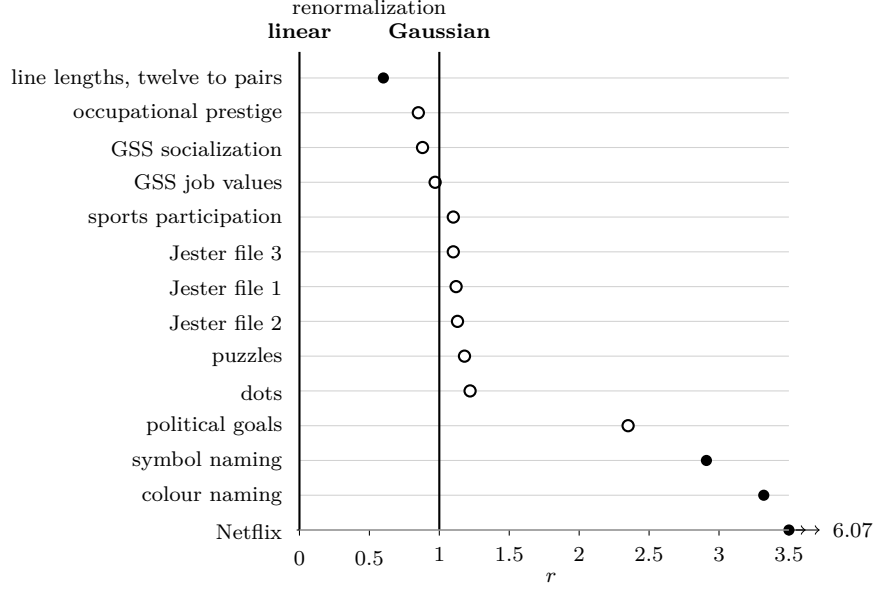
Figure 1: Where each collection sits between the two maps. The coordinate is r = \lambda_{\text{observed}}/\lambda_{\text{Case V}} , the observed contraction slope divided by the slope Case V implies for that collection’s own shares, so linear renormalization is at r = 0 by construction and Gaussian renormalization at r = 1 . Filled circles are restricted menus the observer actually faced; open circles are ranking-induced. Most collections lie beyond r = 1 , so choice contracts by more than Case V predicts and the Gaussian point is not far enough along the family, which is the same signed error the after-stimulus arms and Table 9 report. The one collection on a perceptual continuum falls short of it instead. Positions here do not reproduce the scoreboard: \lambda projects a vector of pair-specific predictions onto a single slope and is not a proper score, so the twelve-line collection sits nearer Case V on this axis while linear renormalization has the lower held-out log loss on it. The axis places populations, Table 1 scores forecasts. Netflix has three alternatives and three pairs.
