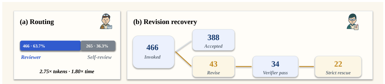
Figure 5. Adaptive Reviewer routing and revision recovery. Panel (a) shows that 466 of 731 tasks invoke an independent Reviewer, while 265 use Engineer self-review; routed tasks consume 2.75\times the solve input Tokens and 1.80\times the active time on average. Panel (b) follows the routed workload: 388 tasks are accepted on first review, 43 receive a revision request, 34 of those later pass the official verifier, and 22 complete the strict review-loop rescue. Routing is task-dependent; a randomized-routing run would additionally isolate the causal effect.
