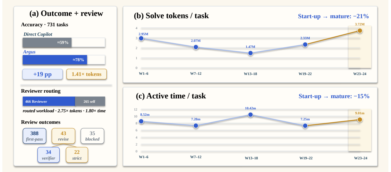
Figure 6. Outcome, review, and longitudinal efficiency in the 731-task SWE-Bench Pro run. Panel (a) reports the full-suite accuracy and aggregate-Token comparison, adaptive Reviewer routing, and observed review outcomes. Panels (b) and (c) aggregate Argus solve input Tokens and active workflow time over approximately six-Wave windows using task-weighted means. Relative to W1–6, W19–22 uses 21% fewer solve input Tokens and 15% less active time per task. Two incomplete Waves are omitted, while W23–24 remains visible as late difficult-task stress. Copilot per-Wave resource traces were not retained; the window comparison characterizes the operating profile over this sequence, and a controlled replay would isolate the learning effect.
