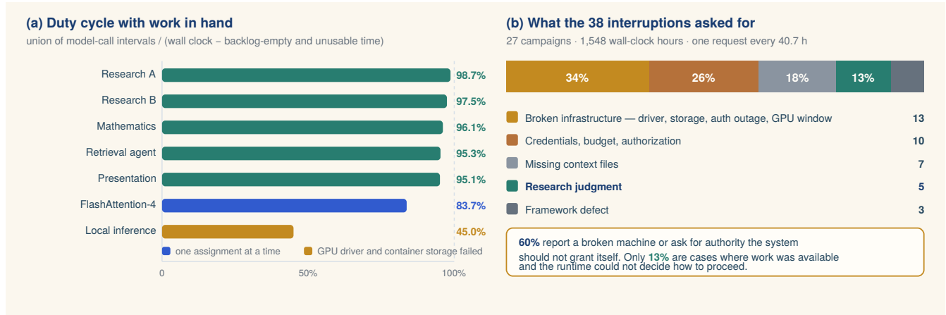
Figure 4. Unattended operating profile. Panel (a) gives duty cycle per campaign under Equation 22; the two lower bars are annotated with why they sit lower, and neither reason is agent hesitation. Panel (b) classifies every human request raised across the 27 campaigns by what it asked for. The two metrics are reported together because neither is interpretable alone: a system that does nothing has a perfect interruption rate, and a system that loops uselessly has a perfect duty cycle.
