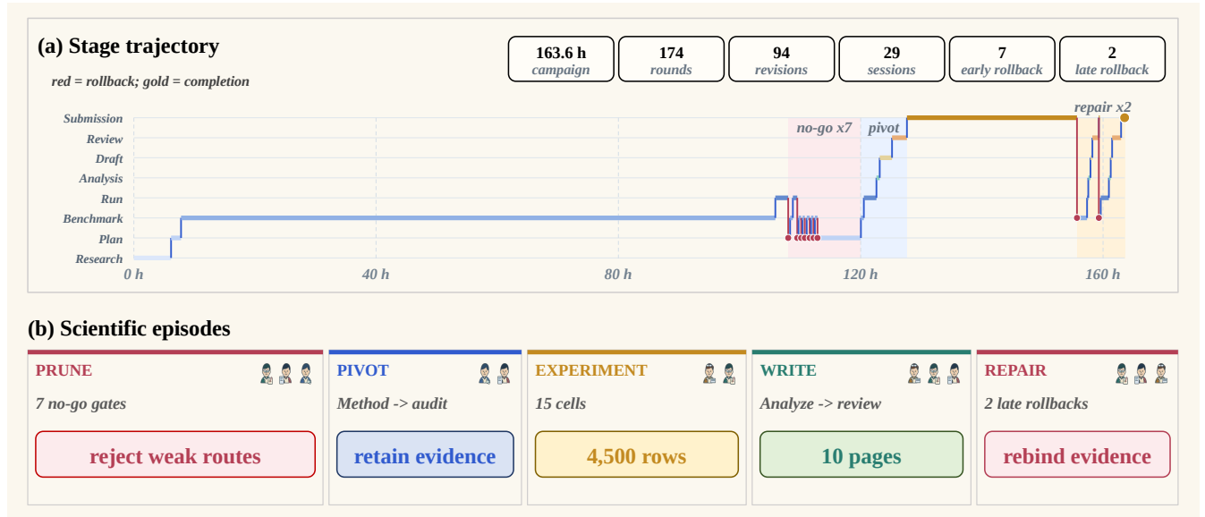
Figure 9. Representative 163.6-hour paper-production trajectory. Panel (a) plots the Manager-controlled Stage against campaign time: seven early approaches were dropped prune weak method routes, the project pivots from a positive method claim to an audit, and two late rollbacks repair the submission evidence. Panel (b) reduces the trace to five scientific episodes—prune, pivot, experiment, write, and repair—while retaining the 15-cell, 4,500-row experiment and the final 10-page manuscript.
