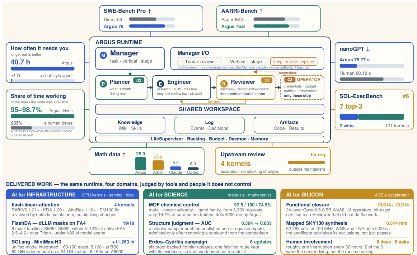
Figure 1. Argus runtime, autonomy profile, and delivered work. The central diagram shows how the three Driver questions are distributed. The Reviewer answers Q1 and runs read-only, so it cannot edit the evidence it judges; its four verdicts include blocked , which withholds completion outright. The Planner answers Q2 under a Manager that holds sole authority over Stage transitions. Q3 is an explicit boundary: credentials, budget, publication, and irreversible actions stop for the operator, while ordinary technical failure does not. The dashed return path is the plan-challenge channel—a Reviewer holding disconfirming evidence may mark the plan for reconsideration, and the Manager decides whether to keep, revise, or replace it, which prevents an early decision from binding better-informed rounds (Section 7.6). All roles operate over a shared workspace whose knowledge, event log, artifacts, backlog, budget, daemon, and memory persist across bounded missions. The cards immediately surrounding it report task-native benchmark outcomes together with the two measurements of unattended operation: how long the runtime goes before it needs a person, and what share of its available time it spends producing. The human-driven comparison on the second card is arithmetic rather than a measured system: a harness cannot outlast its operator’s working day, which bounds it near a third of wall-clock time however capable its model becomes. Bars use independent scales and indicate comparison direction with arrows; they are breadth evidence rather than a single normalized leaderboard. The lower band summarizes delivered work in three domains where the deciding evaluator is external to the runtime: a compiler and a reference implementation for infrastructure, an independent chemistry validator and a proof checker for science, and a static-timing engine for silicon. The silicon card also records the human cost of that campaign—eight days, six interruptions, two of them caused by the server failing rather than by the runtime asking.
