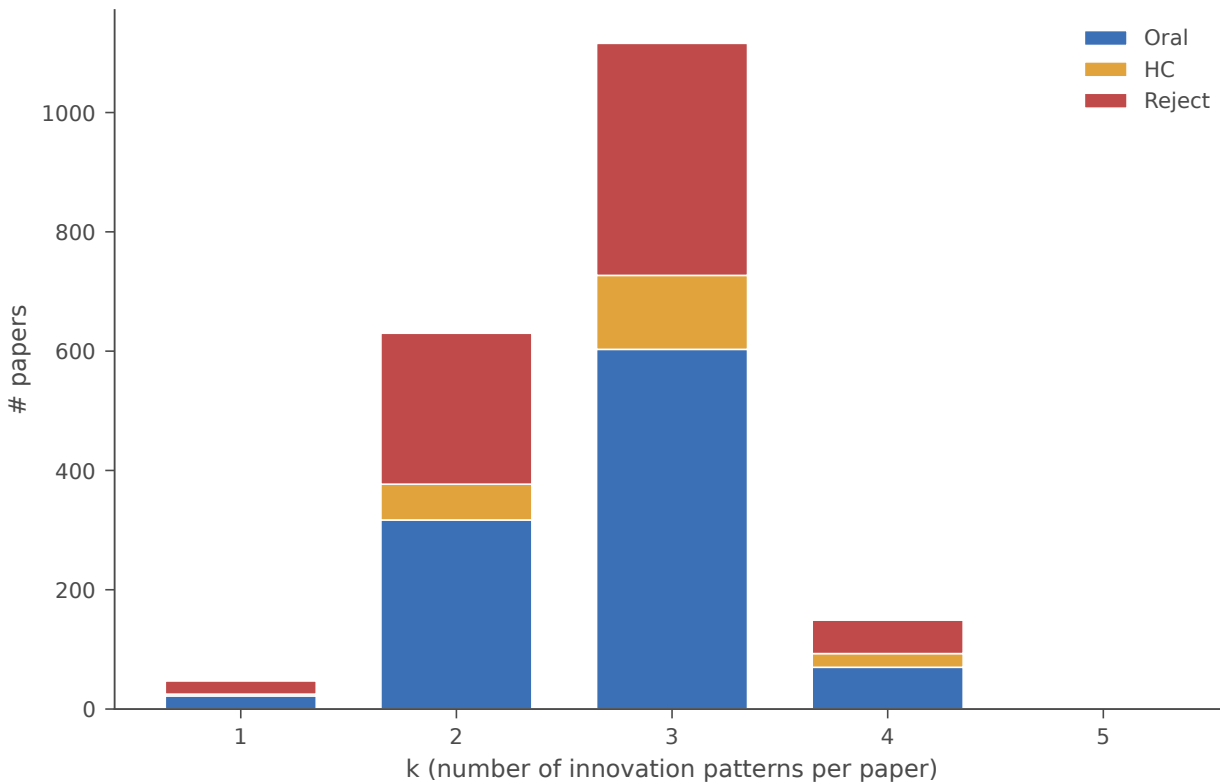
(a) k distribution, stacked counts by acceptance class
