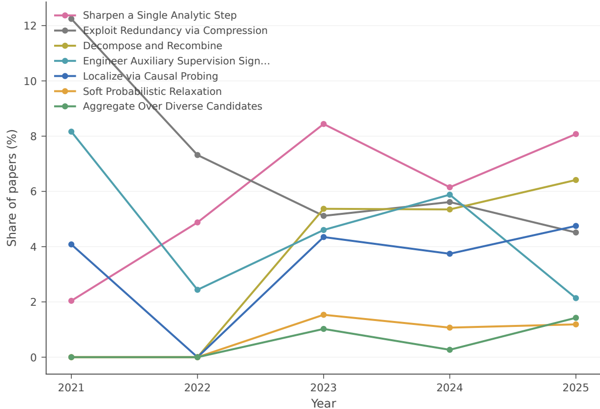
Remaining 7 innovation patterns
