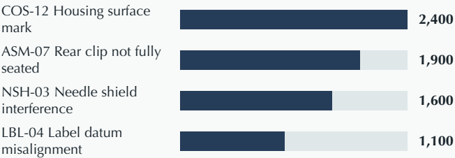
Figure 1. Defect Pareto by quantity
