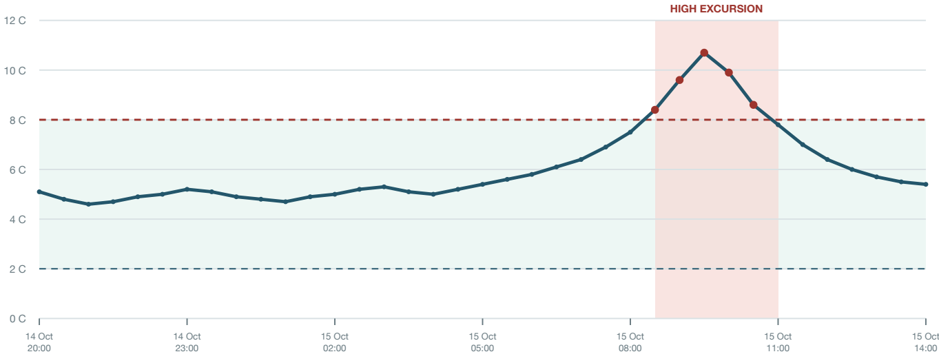
Temperature profile All times UTC | Validated range 2.0-8.0 C
