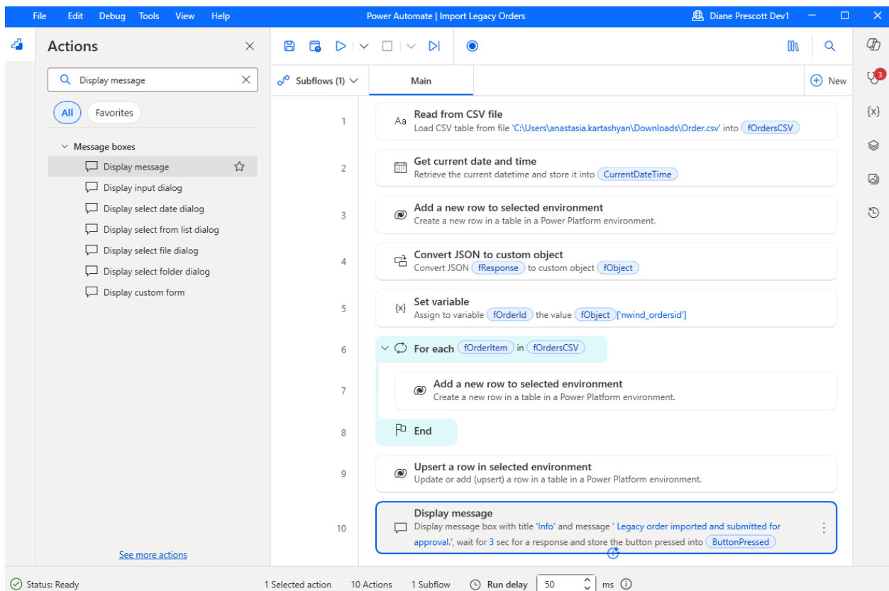
Figure: The end-to-end desktop flow.
