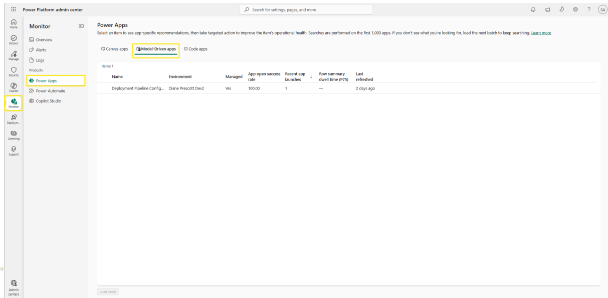
Figure: Monitor Power Apps page with the app tabs and health columns.
