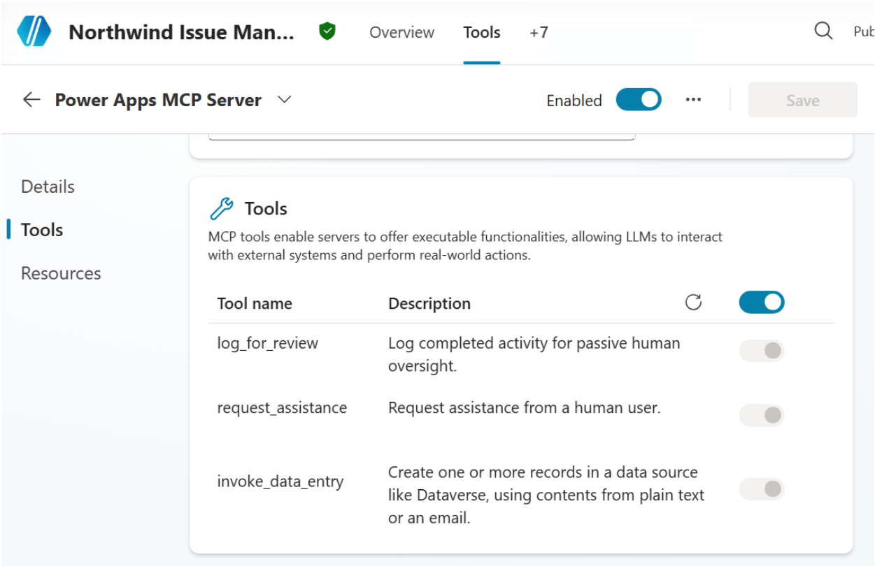
Figure: Power Apps MCP Tools.
