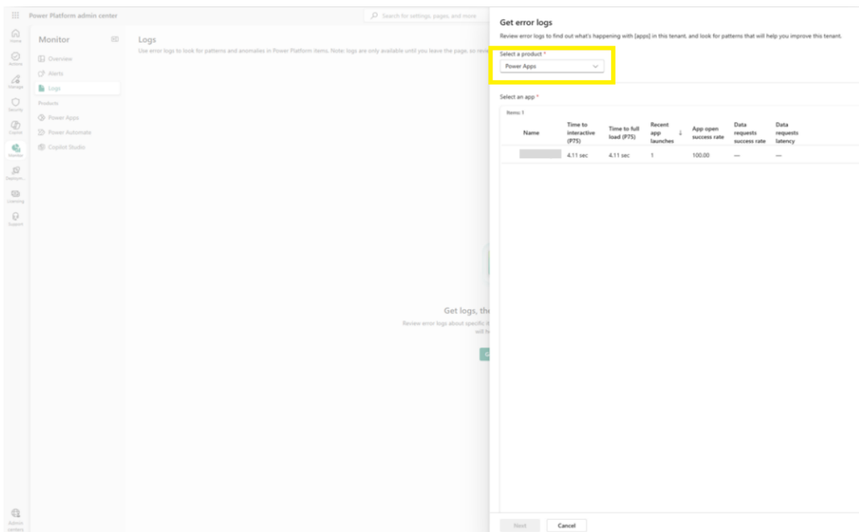
Figure: Get error logs panel with the product dropdown and app list.
