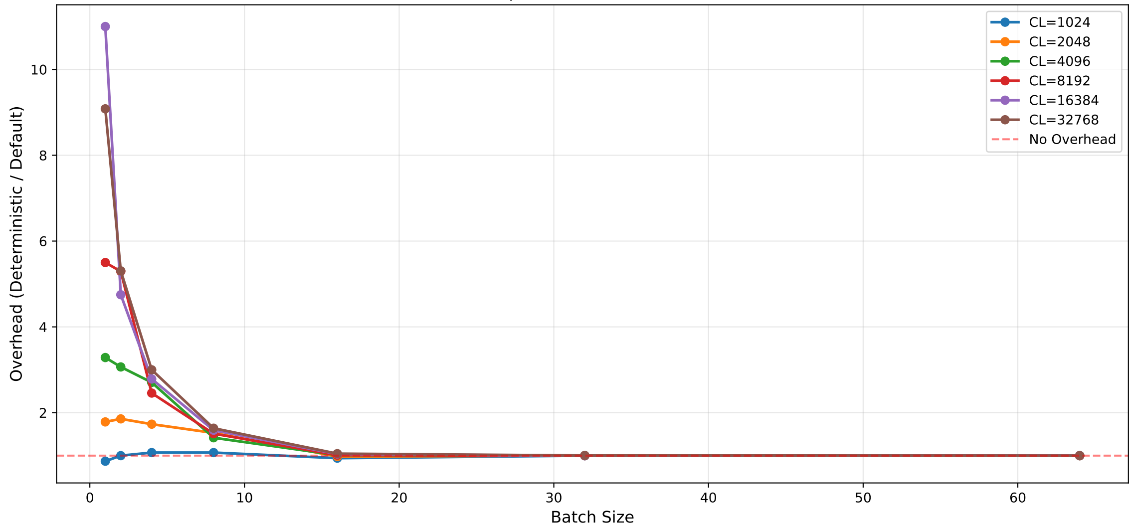
llama-8b-tp2 - Deterministic Overhead
