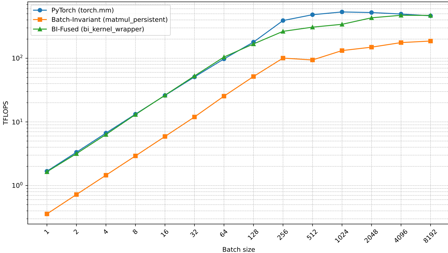
TFLOPS vs Batch size - mlp_down (MLP Down Projection), H100-PCle, bf16
