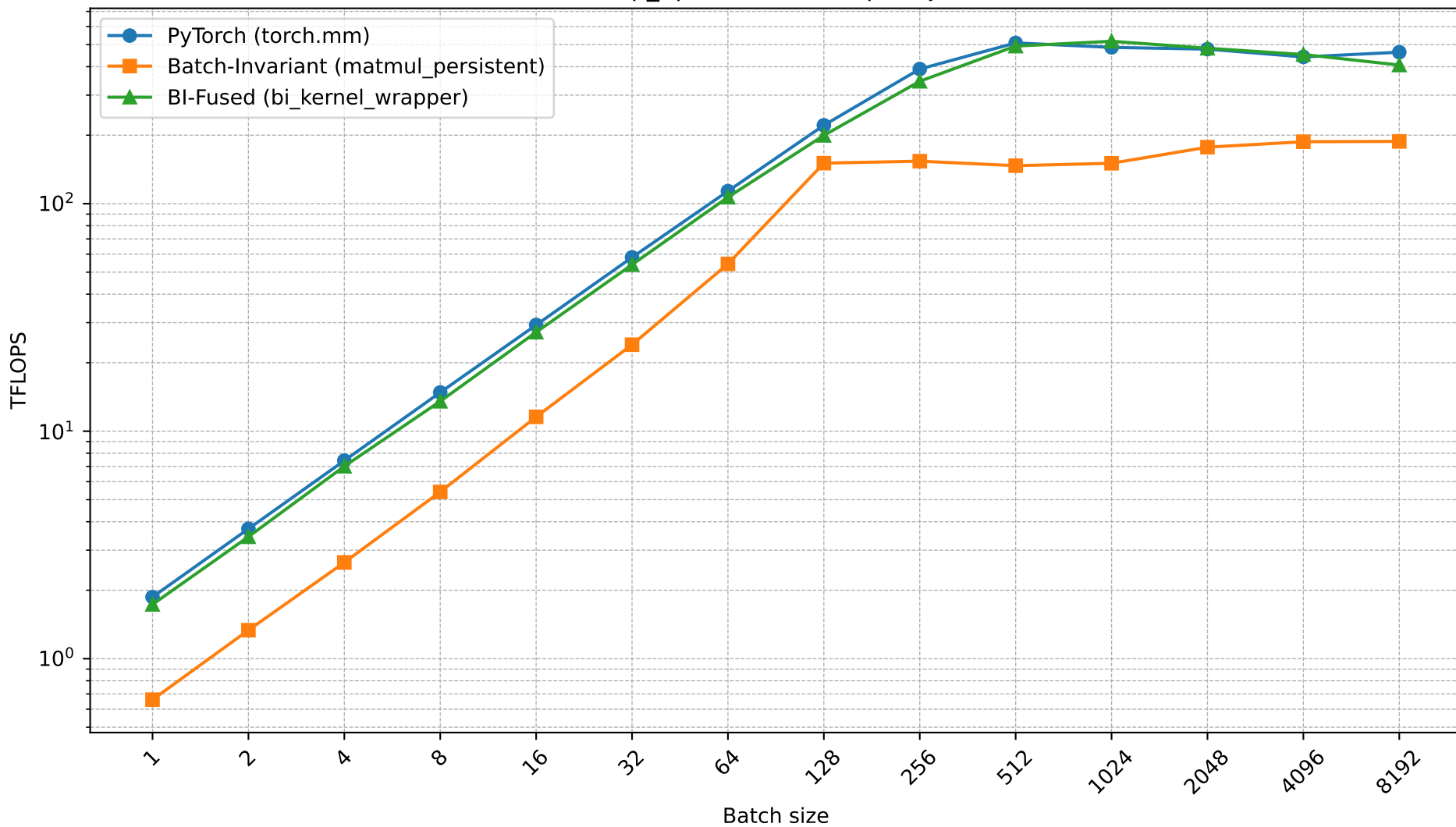
TFLOPS vs Batch size - mlp_up (MLP Gate+Up Projection), H100-PCIe, bf16
