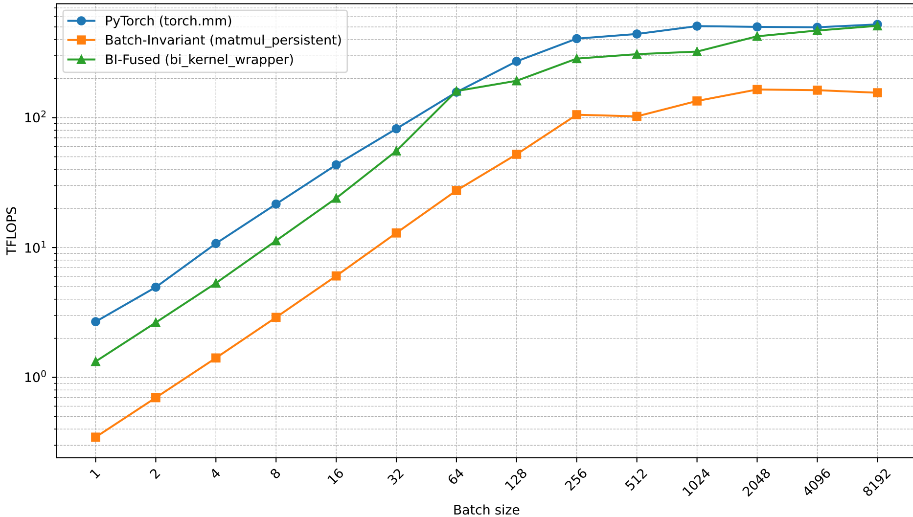
TFLOPS vs Batch size - postproj (Attention O Projection), H100-PCIe, bf16
