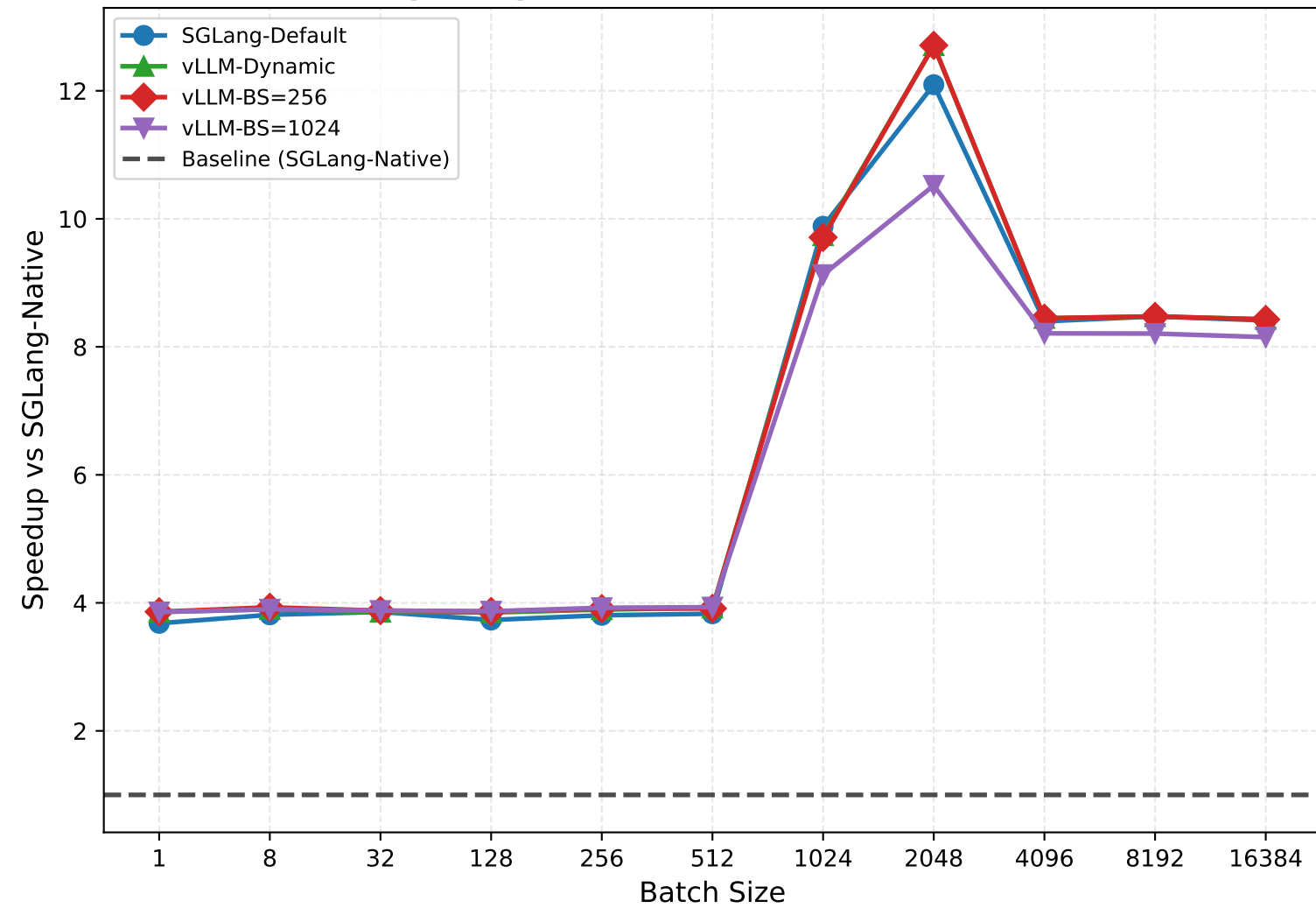
Speedup vs Native - Hidden Size 8192
