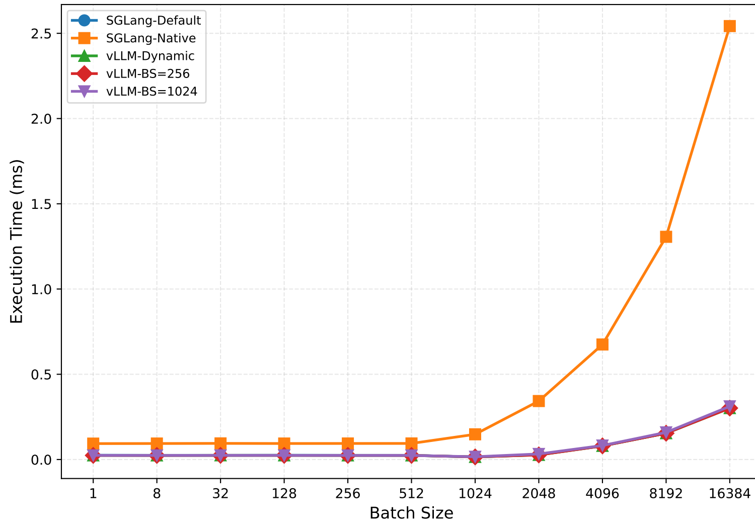
Raw Execution Time - Hidden Size 8192
