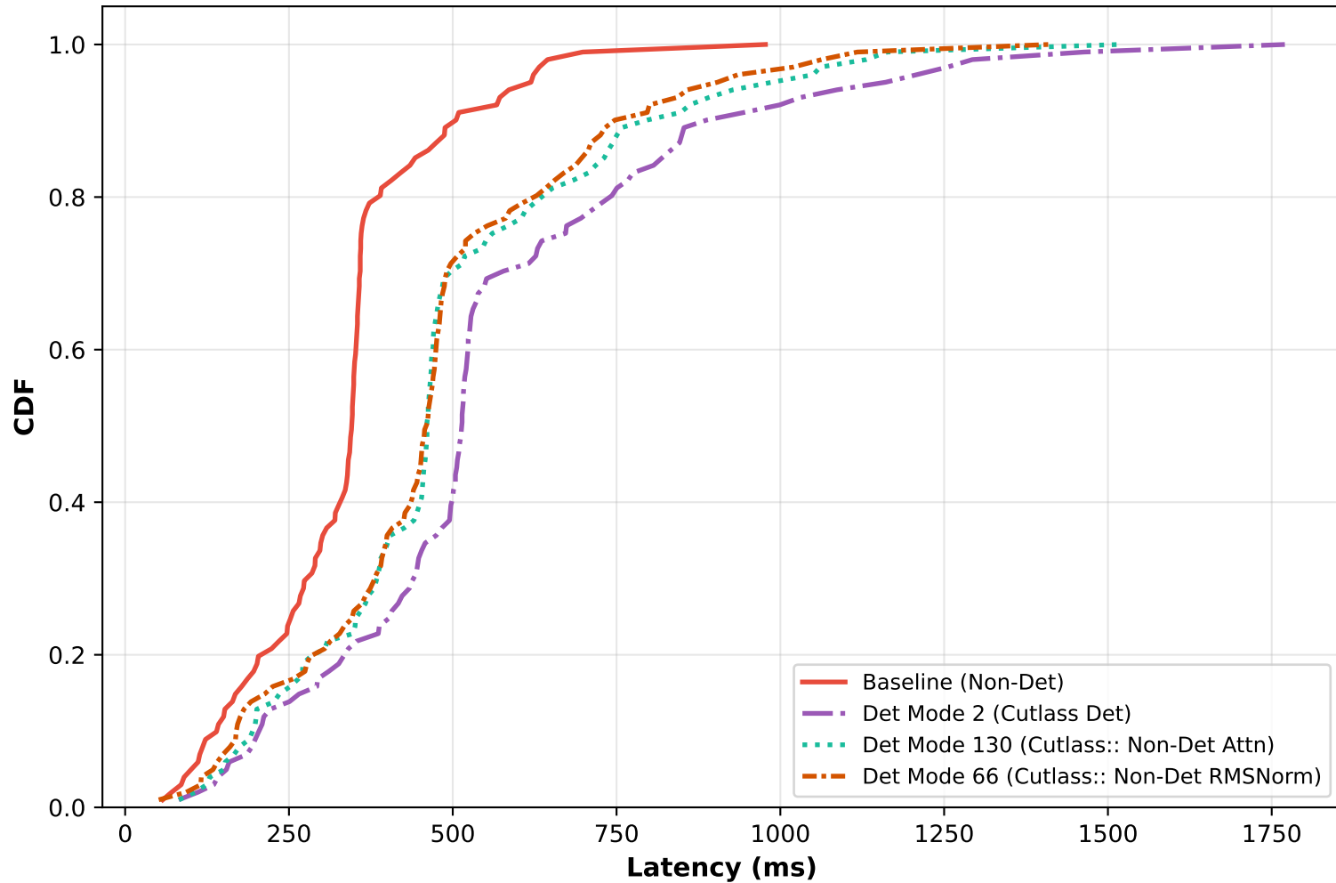
Cutlass-Based
