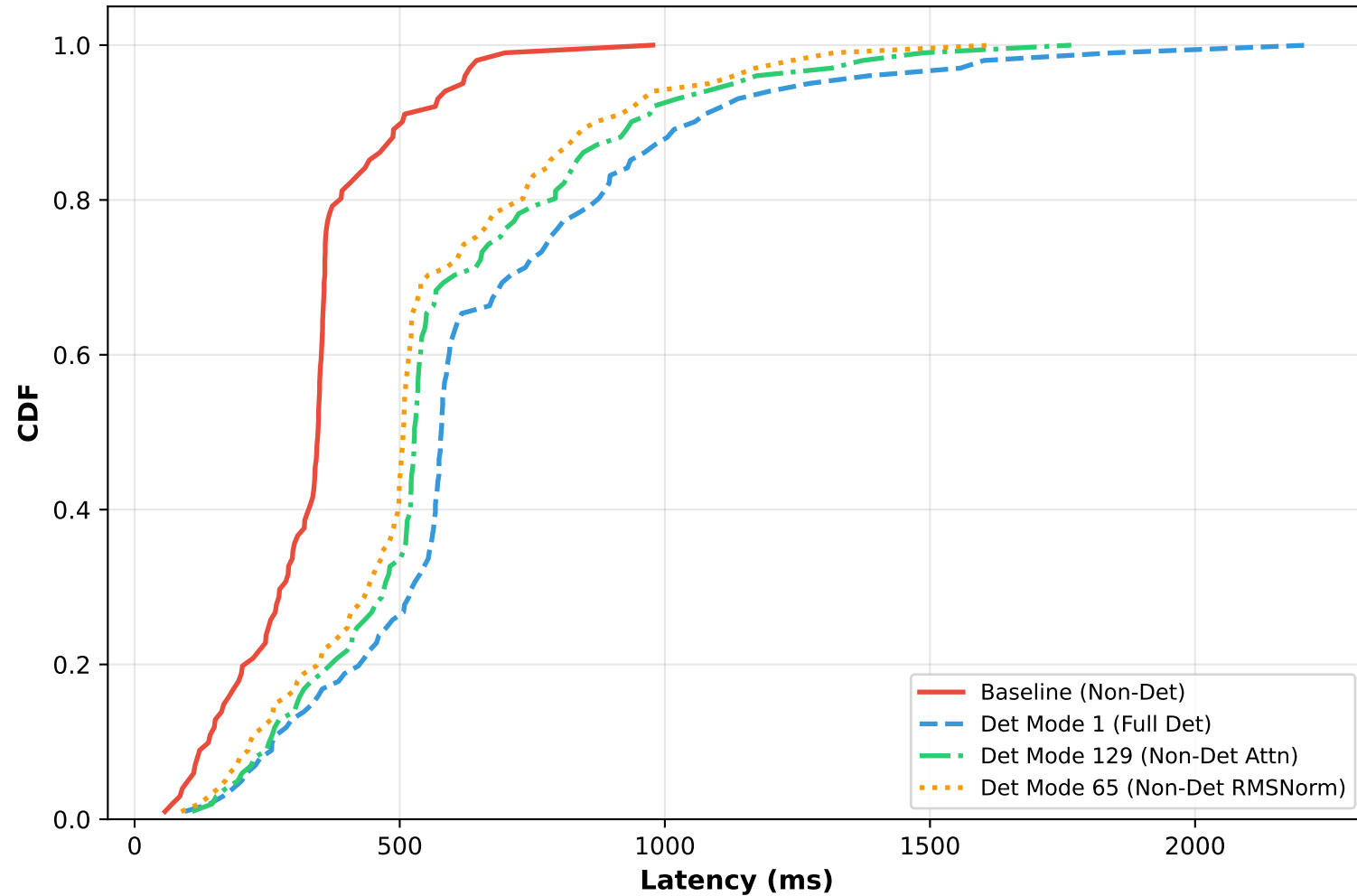
Thinking Machine
