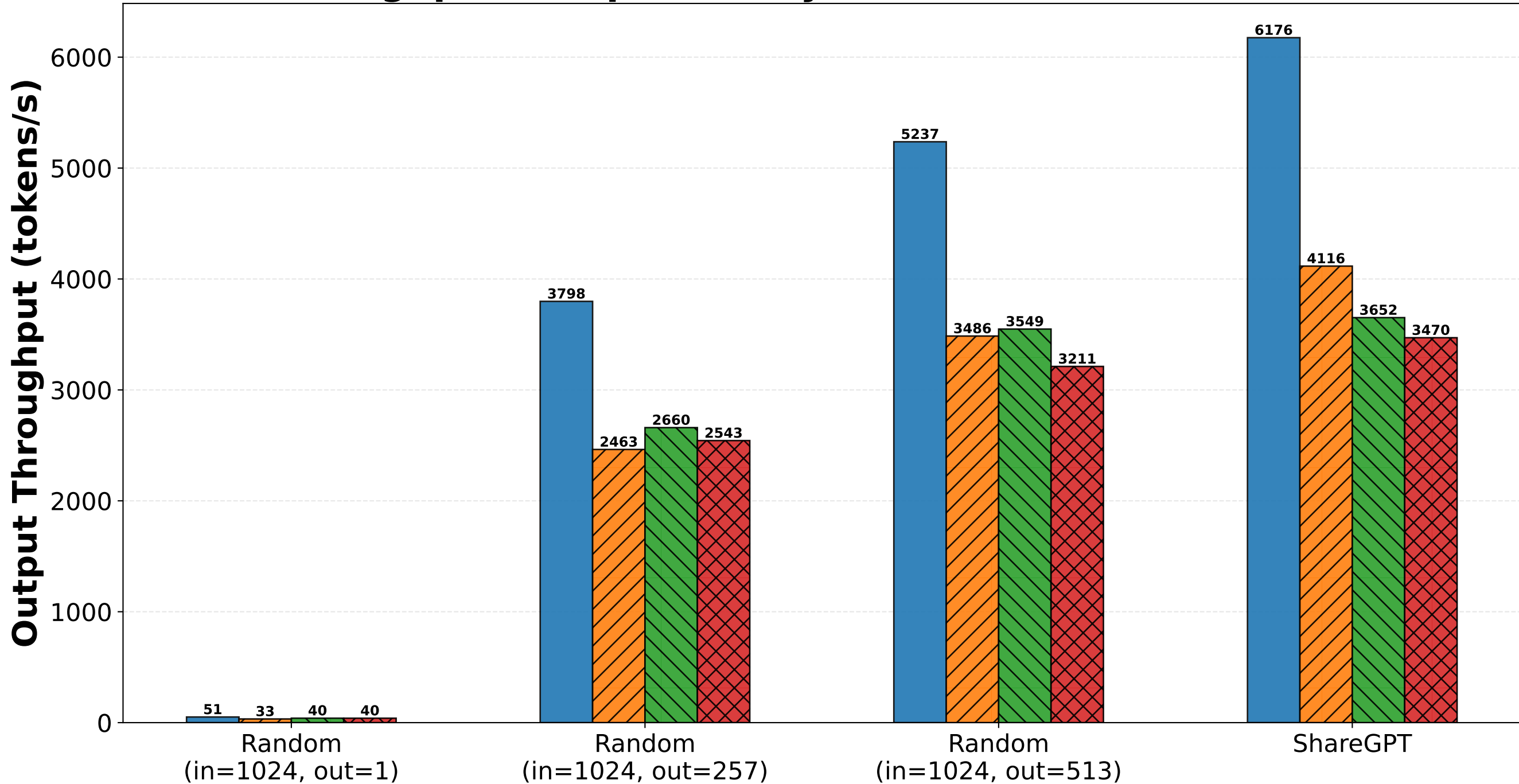
Non-Det Global-Det DetInfer-ws32-bs16 DetInfer-ws64-bs16 Throughput Comparison by Dataset (Det Ratio=100%)
