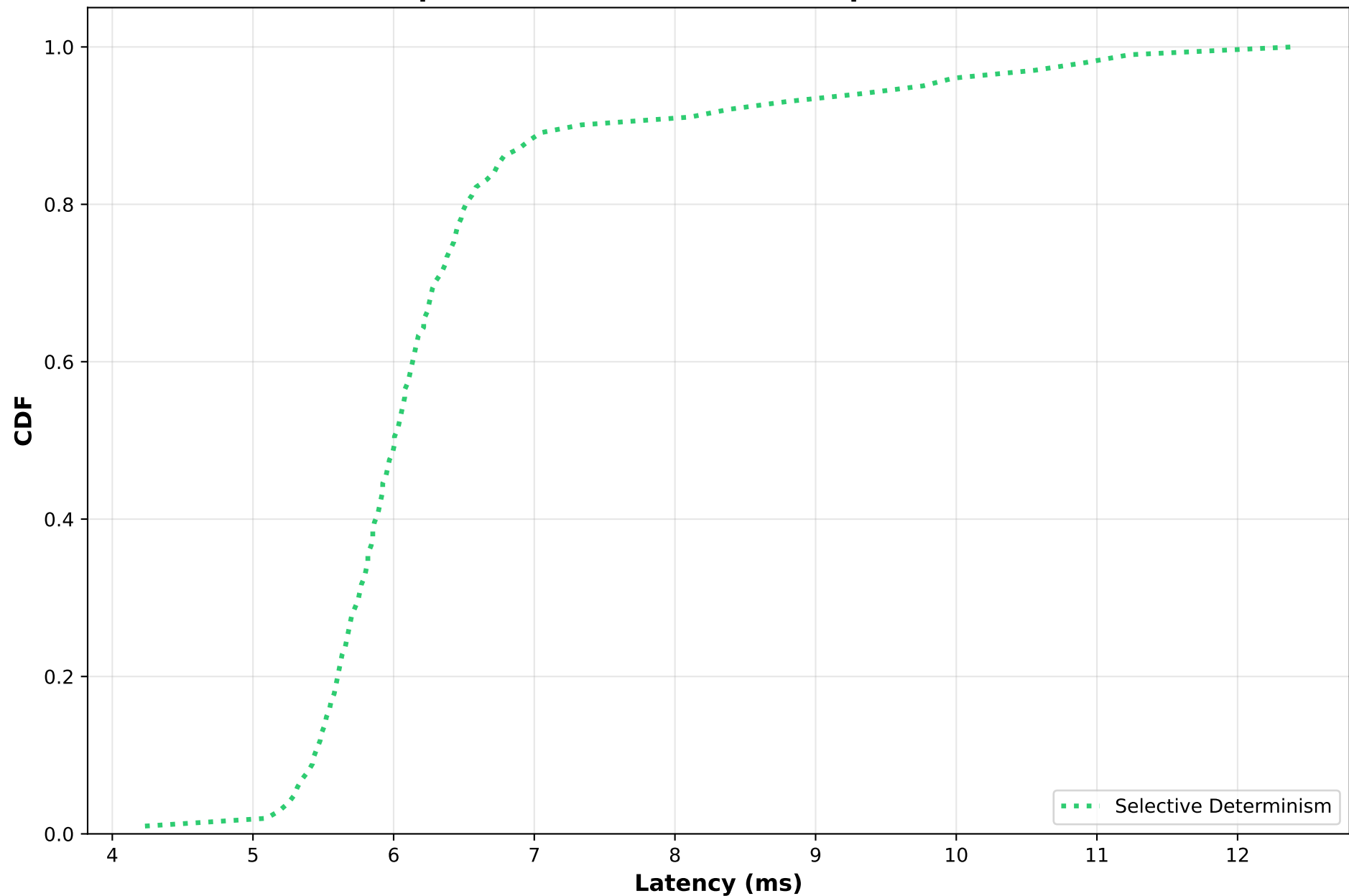
Mixed Temperature Test - Time Per Output Token (TPOT) CDF
