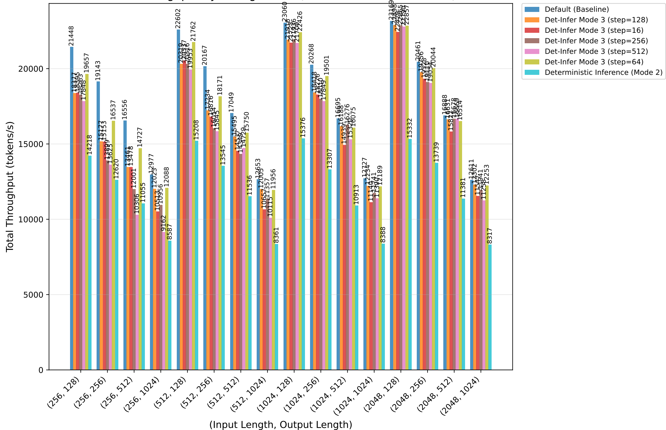
Total Throughput by Configuration (Deterministic Ratio = 0.02)
