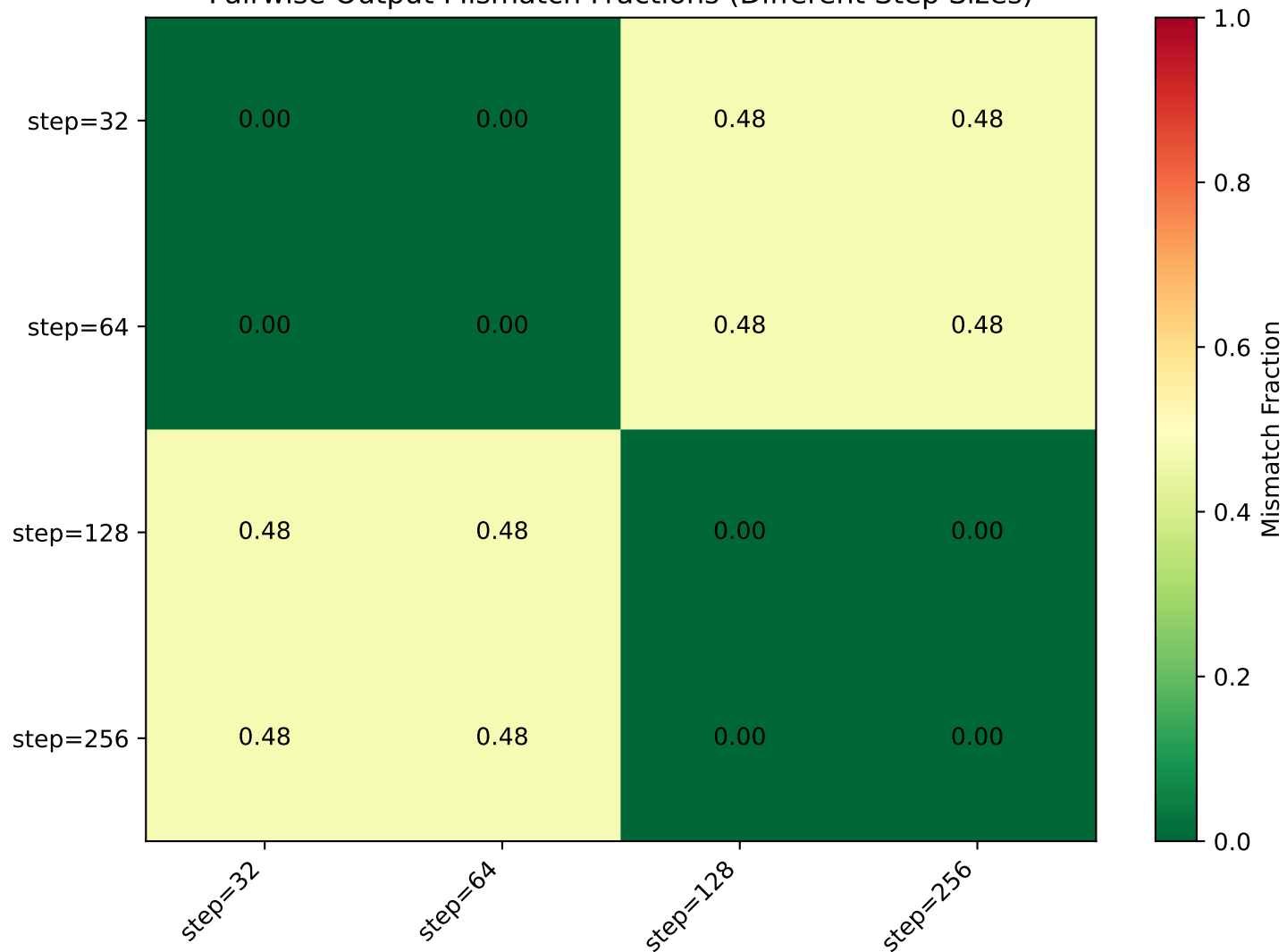
Pairwise Output Mismatch Fractions (Different Step Sizes)
