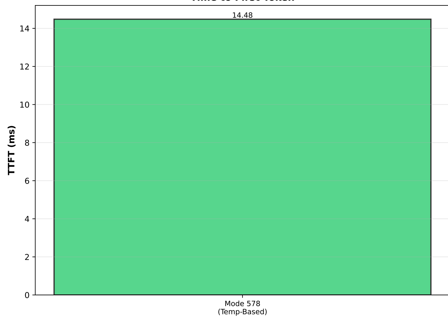
Mixed Temperature Test - Performance Summary (Mean Values) Metric Value Output Throughput 66.8 Time to First Token 14.48 Time Per Output Token 144.380 End-to-End Latency 6719.1
