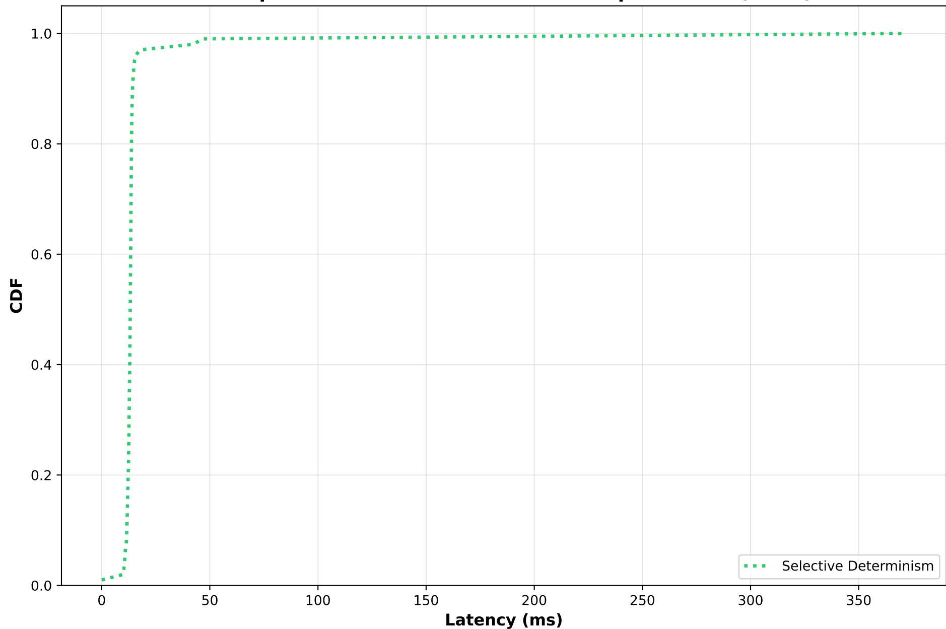
Mixed Temperature Test - Time Between Output Tokens (TBOT) CDF
