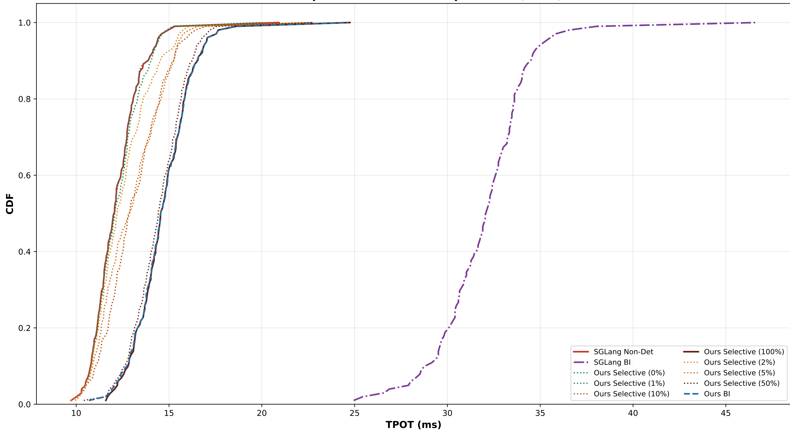
Unified Comparison - Time Per Output Token (TPOT) CDF
