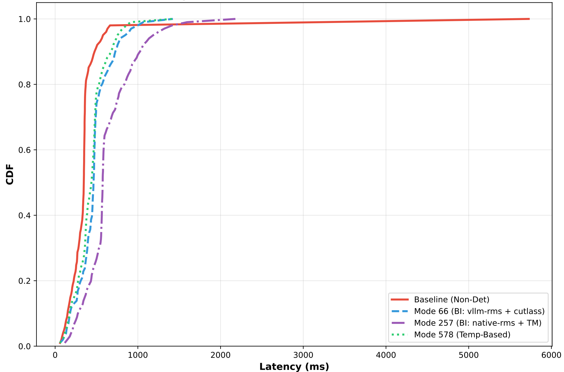
Mixed Temperature Test - Time to First Token (TTFT) CDF
