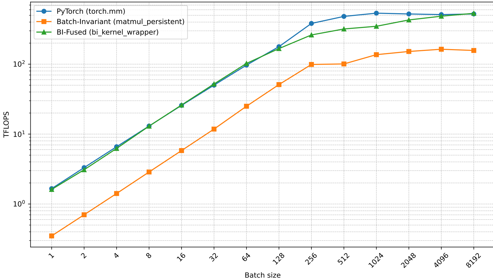
TFLOPS vs Batch size - mlp_down (MLP Down Projection), H100-PCIe, bf16
