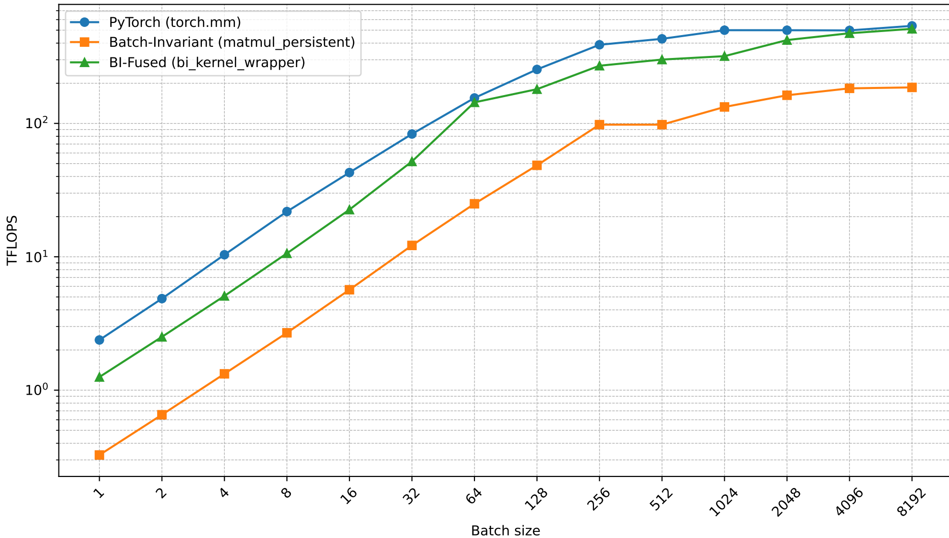
TFLOPS vs Batch size - preproj (Attention Q/K/V Projection), H100-PCIe, bf16
