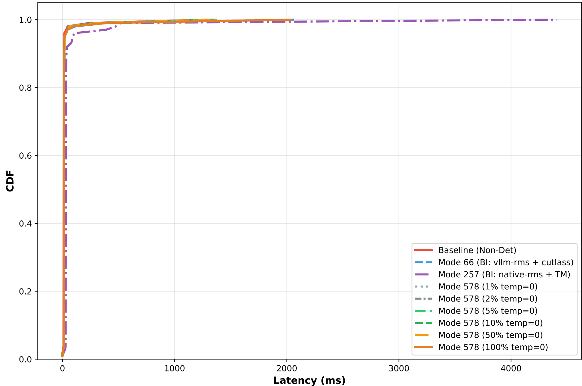
Component Test - Time Between Output Tokens (TBOT) CDF
