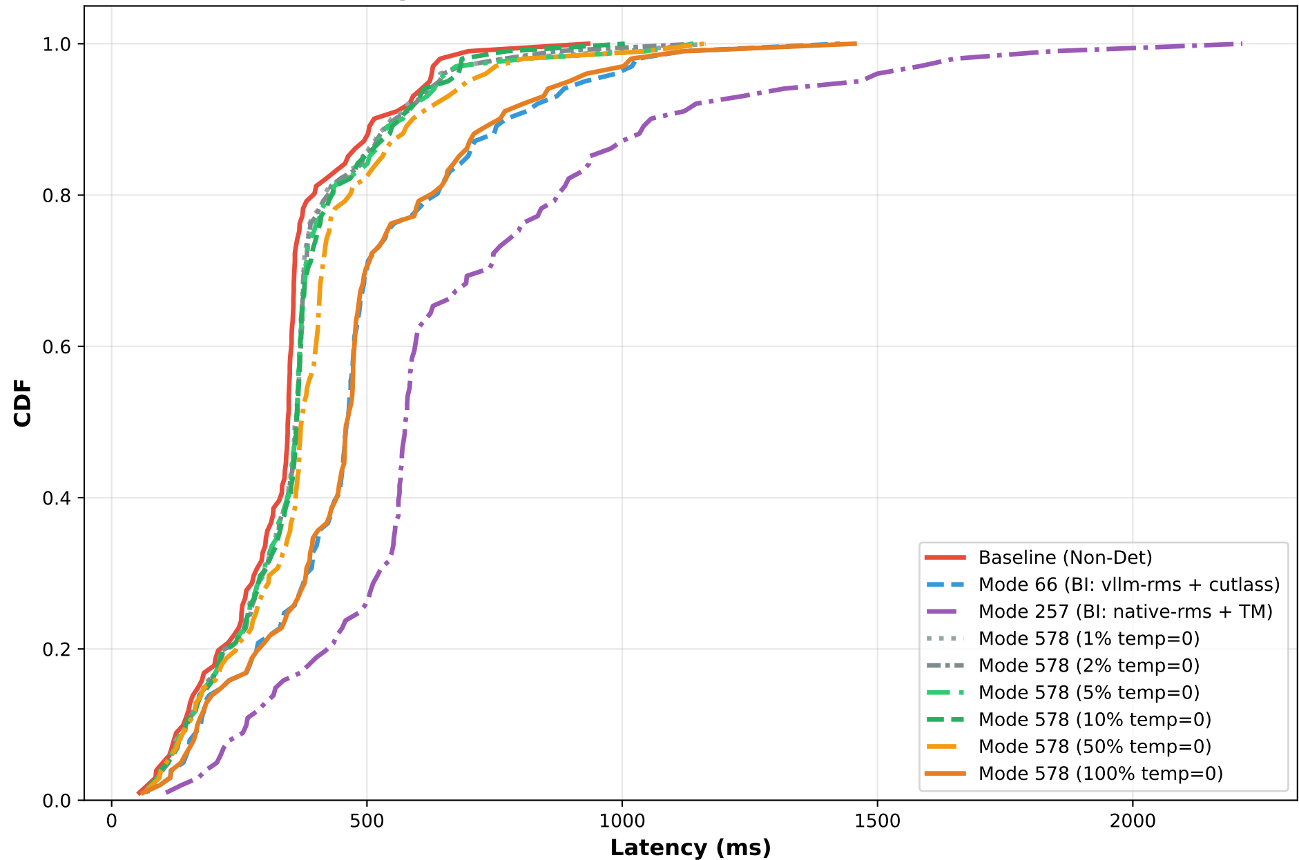
Component Test - Time to First Token (TTFT) CDF
