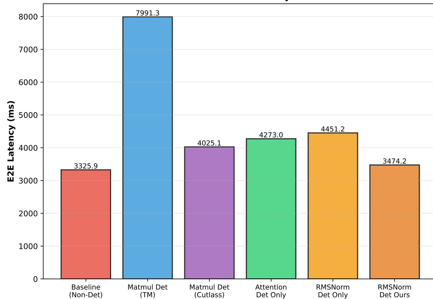
End-to-End Latency
