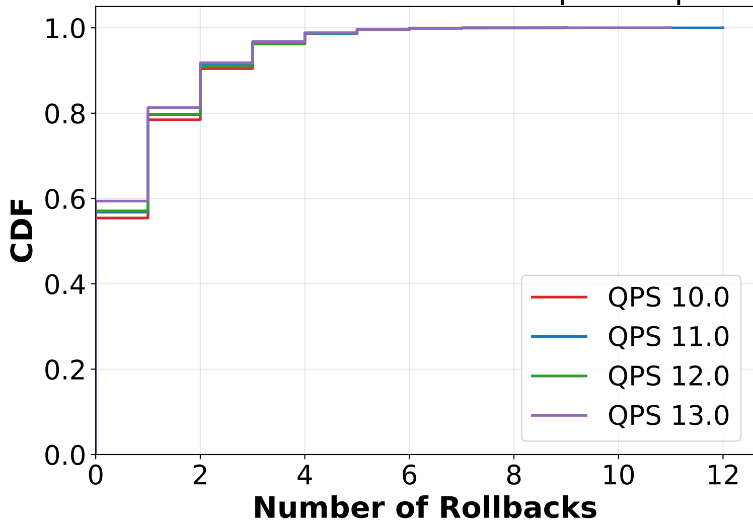
CDF of Number of Rollbacks per Request
