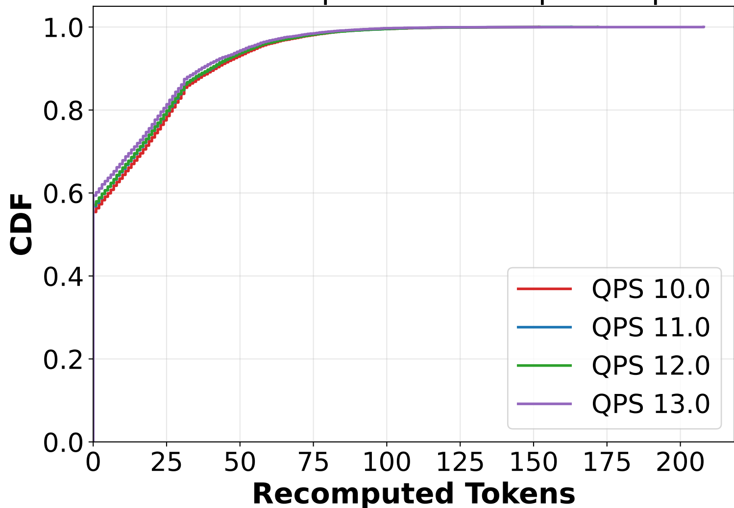
CDF of Recomputed Tokens per Request
